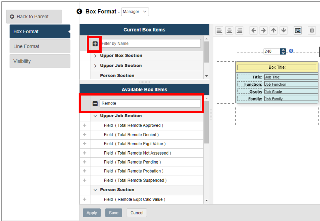
Figure 4: Filter on Current and Available Box Items
